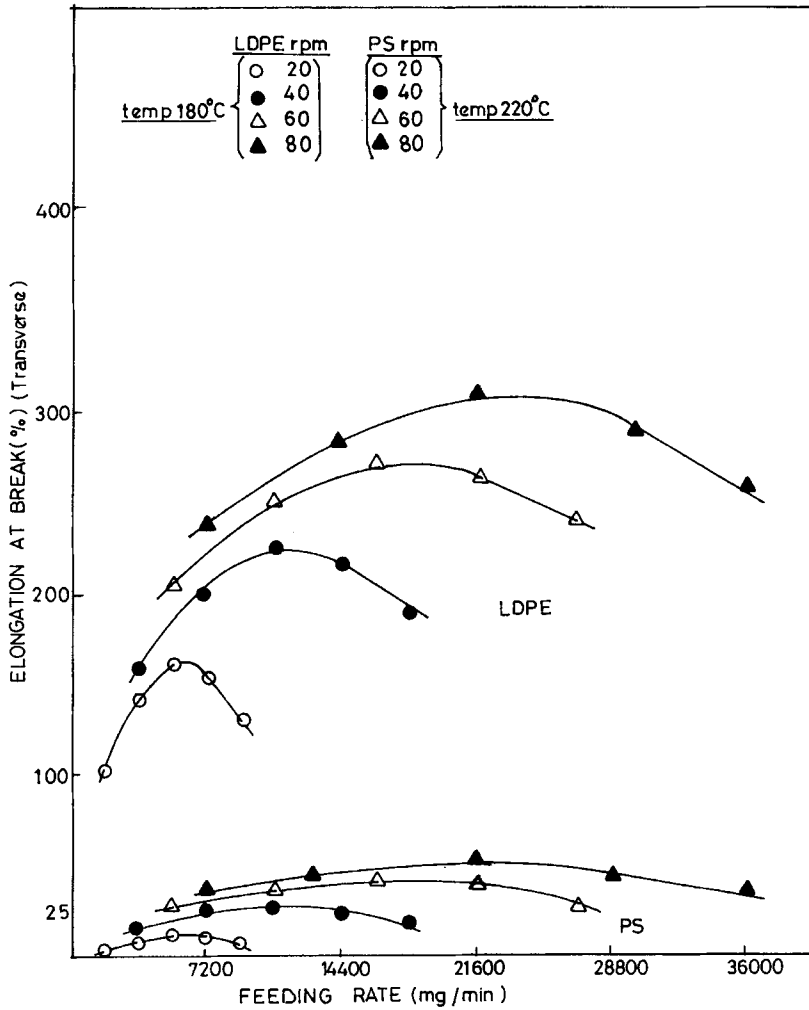
FIGURE 6 Effect of feeding rate on the elongation at break of LDPE and PS at different rpms in transverse direction.
