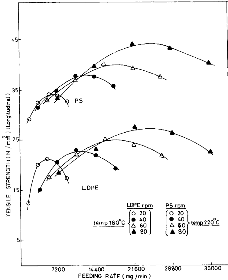
FIGURE 3 Effect of feeding rate on the tensile strength of LDPE and PS at different rpm in longitudinal (extrusion) direction.
