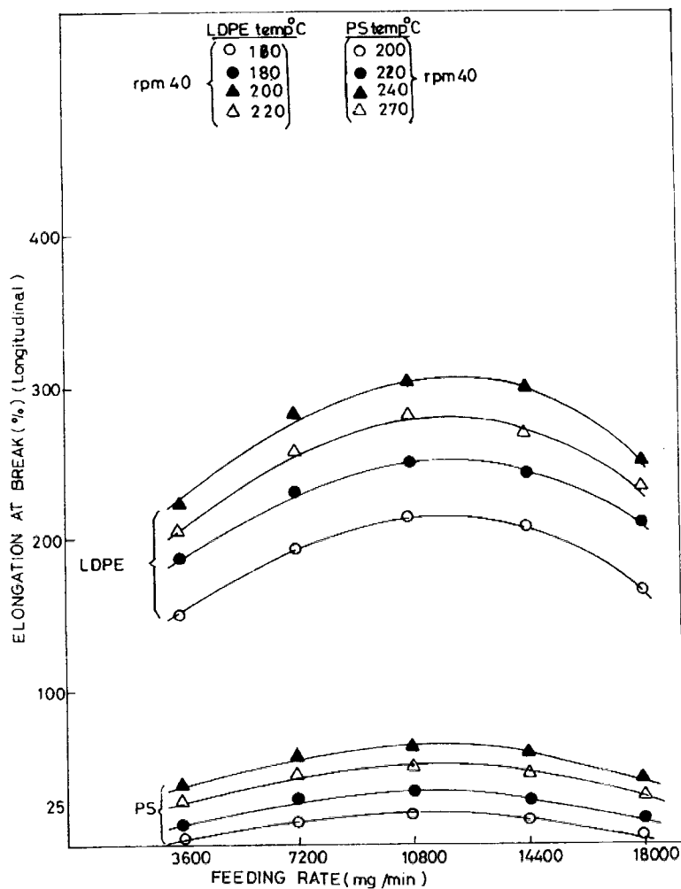
FIGURE 9 Effect of feeding rate on the elongation at break of LDPE and PS at different temperatures in longitudinal (extrusion) direction.
